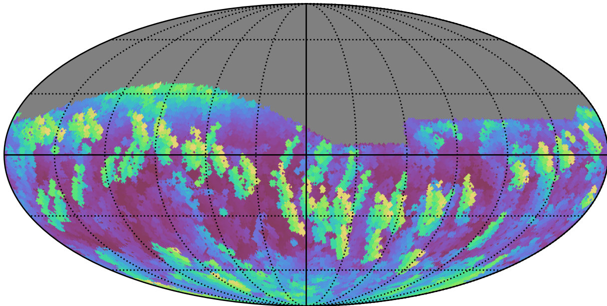
smc_lmc_v3.3_10yrs Yr 1 i band: Max airmass
