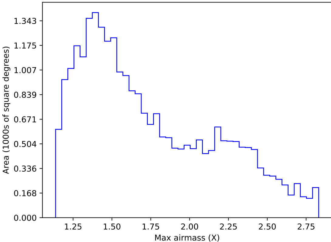
smc_lmc_v3.3_10yrs Yr 1 i band: Max airmass
