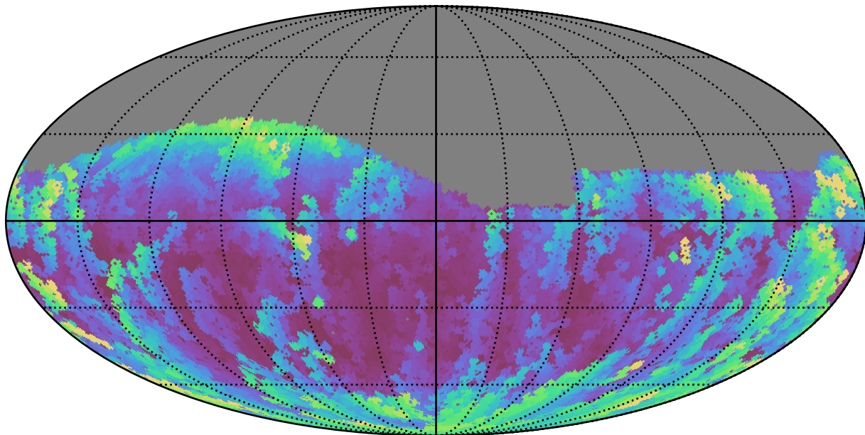
smc_lmc_v3.3_10yrs Yr 1 g band: Max airmass
