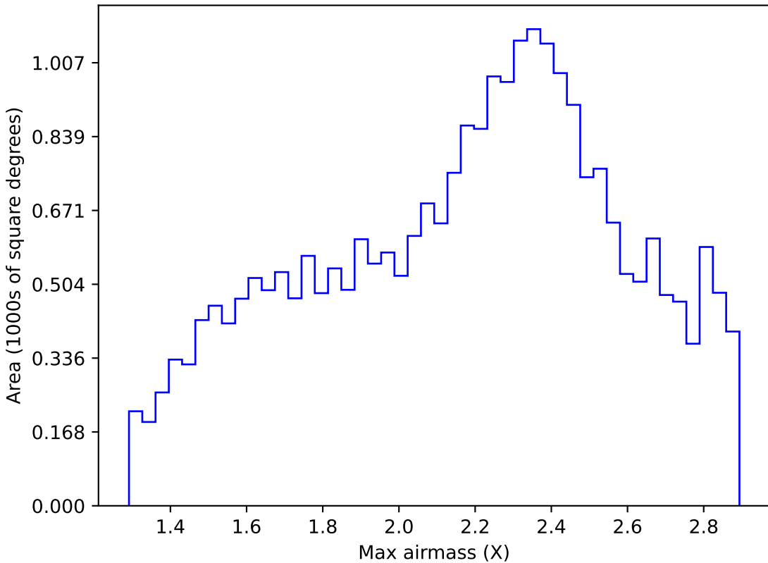
smc_lmc_v3.3_10yrs Yr 1 all bands: Max airmass
