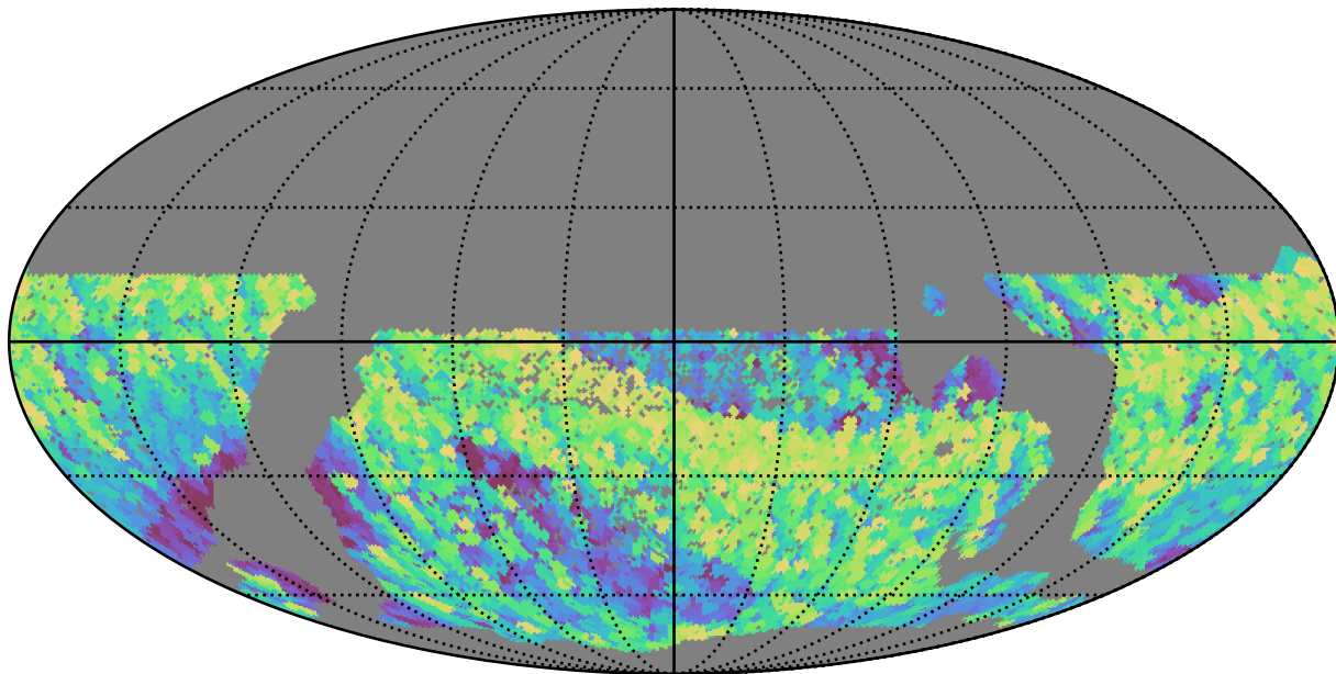
smc_lmc_v3.3_10yrs WFD z band: Max airmass
