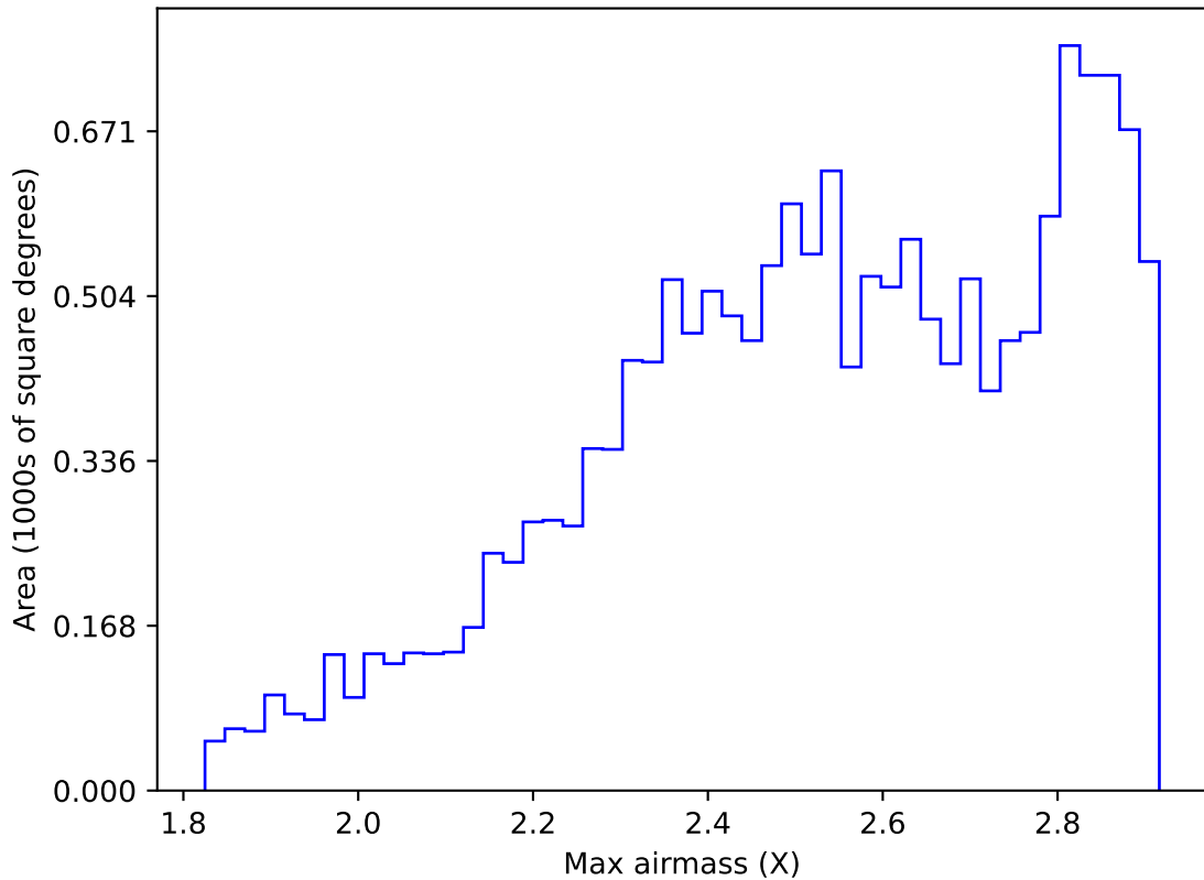
smc_lmc_v3.3_10yrs WFD z band: Max airmass
