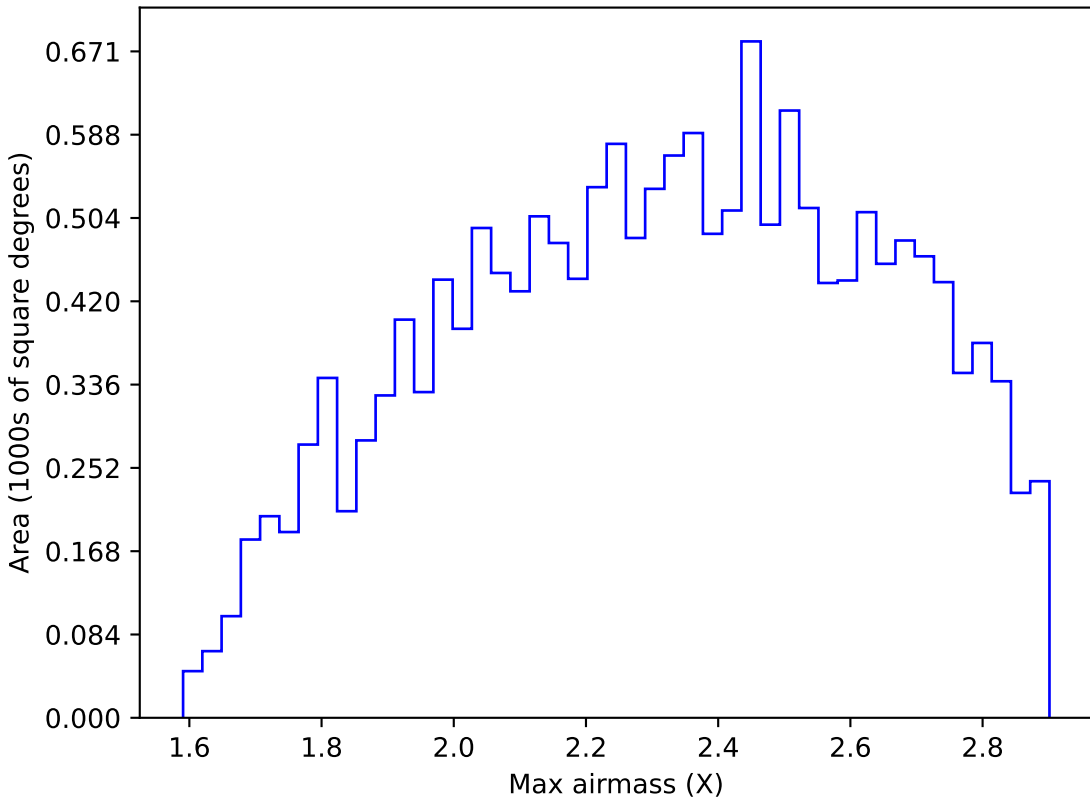
smc_lmc_v3.3_10yrs WFD y band: Max airmass
