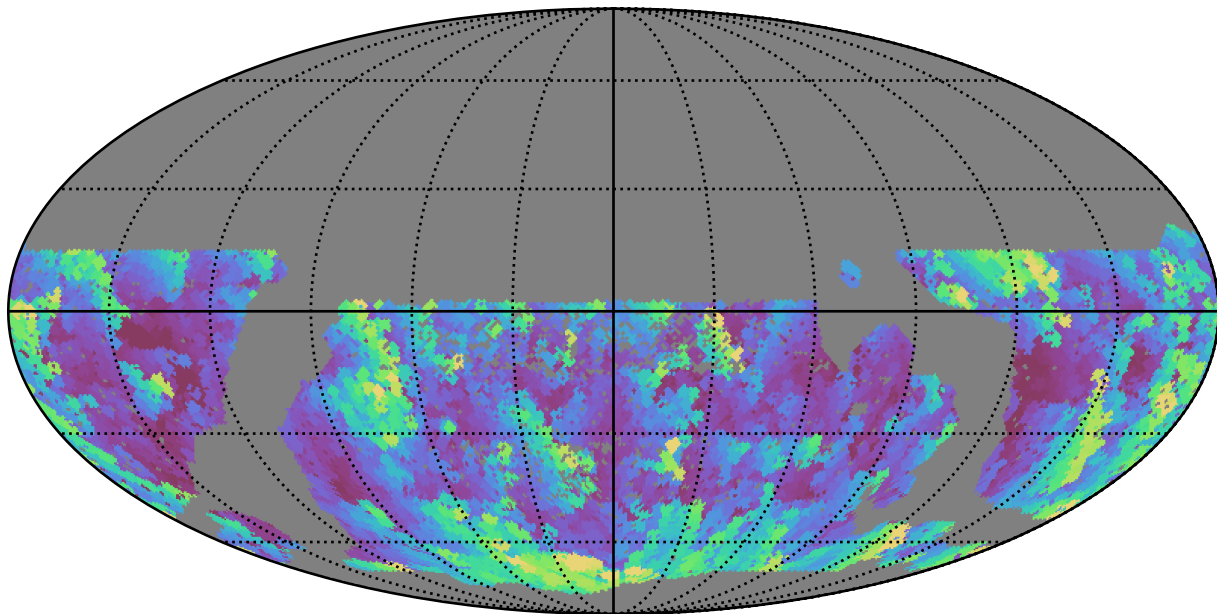
smc_lmc_v3.3_10yrs WFD u band: Max airmass
