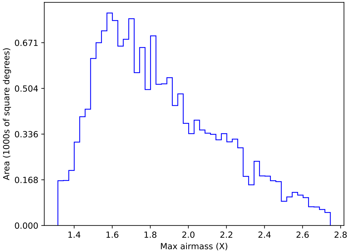
smc_lmc_v3.3_10yrs WFD u band: Max airmass
