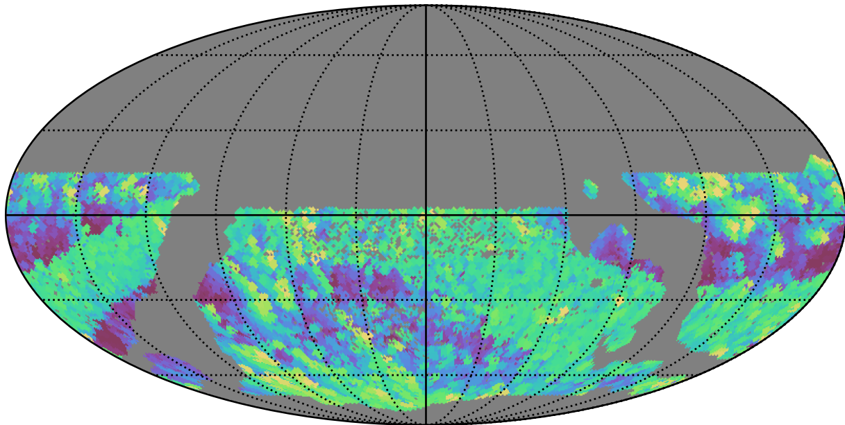
smc_lmc_v3.3_10yrs WFD r band: Max airmass
