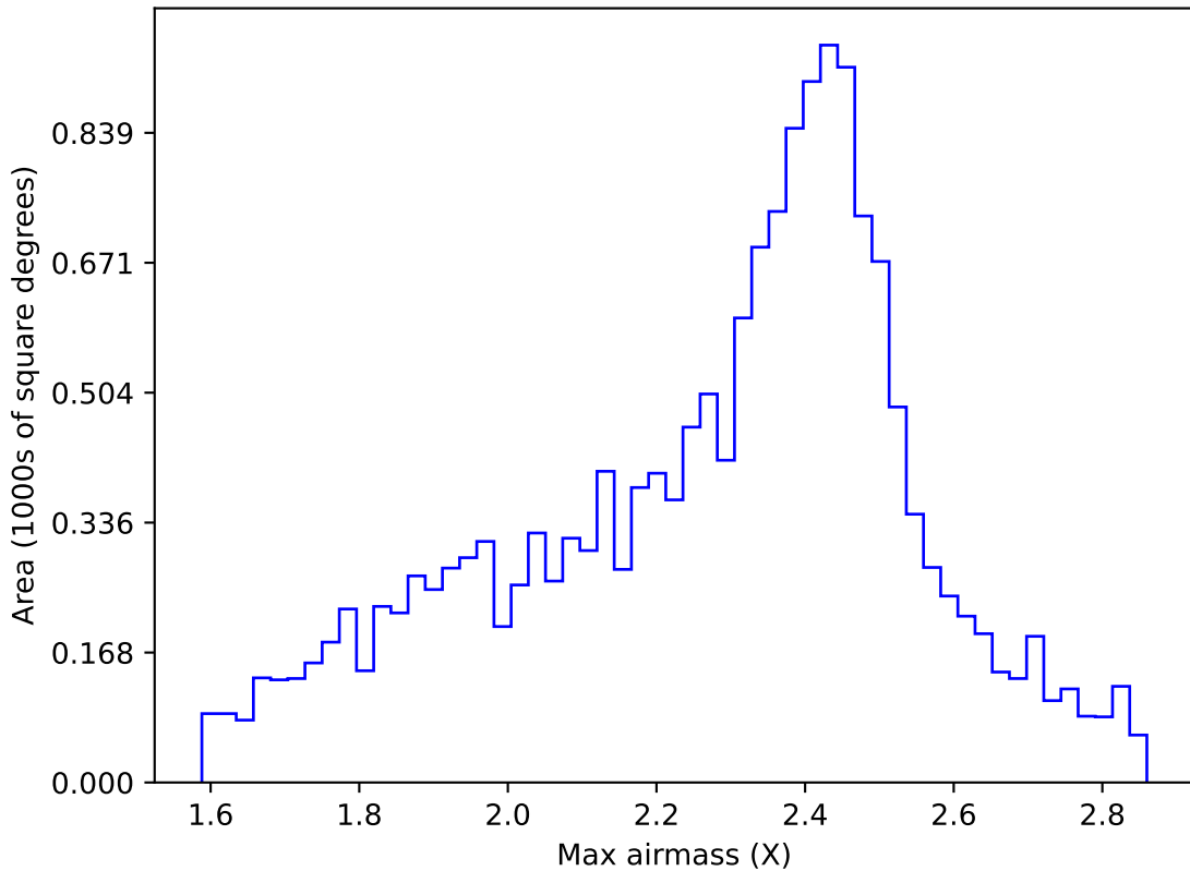
smc_lmc_v3.3_10yrs WFD r band: Max airmass
