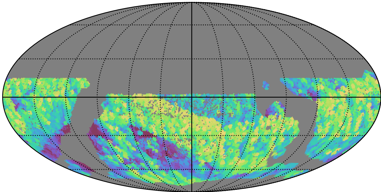
smc_lmc_v3.3_10yrs WFD i band: Max airmass
