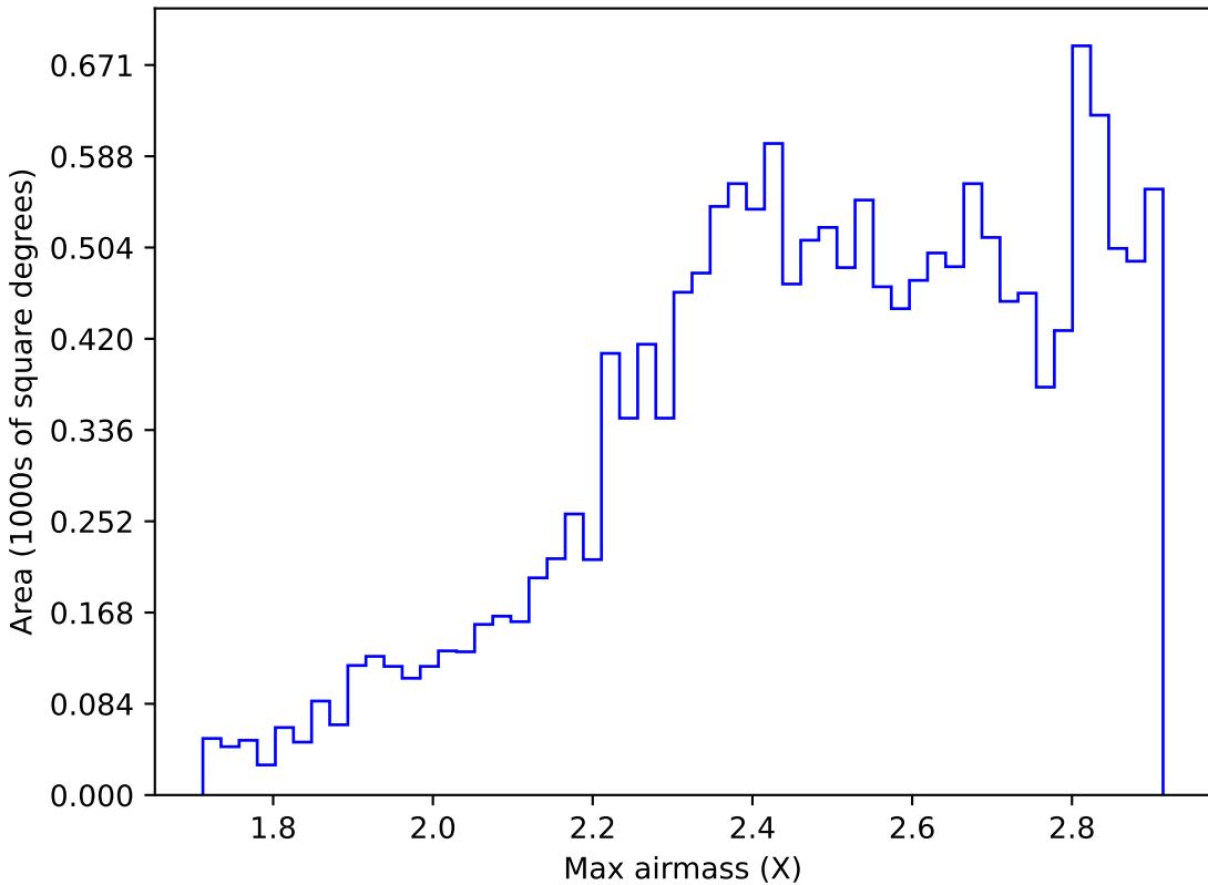
smc_lmc_v3.3_10yrs WFD i band: Max airmass
