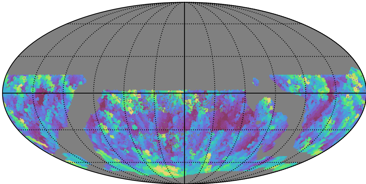
smc_lmc_v3.3_10yrs WFD g band: Max airmass
