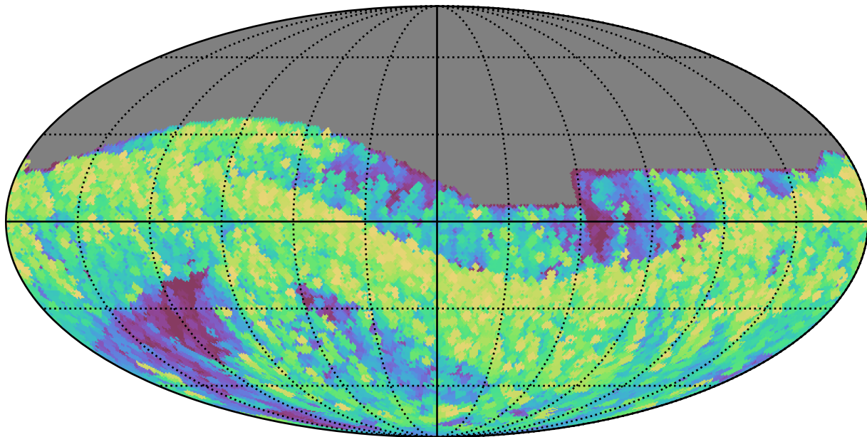
smc_lmc_v3.3_10yrs All sky z band: Max airmass
