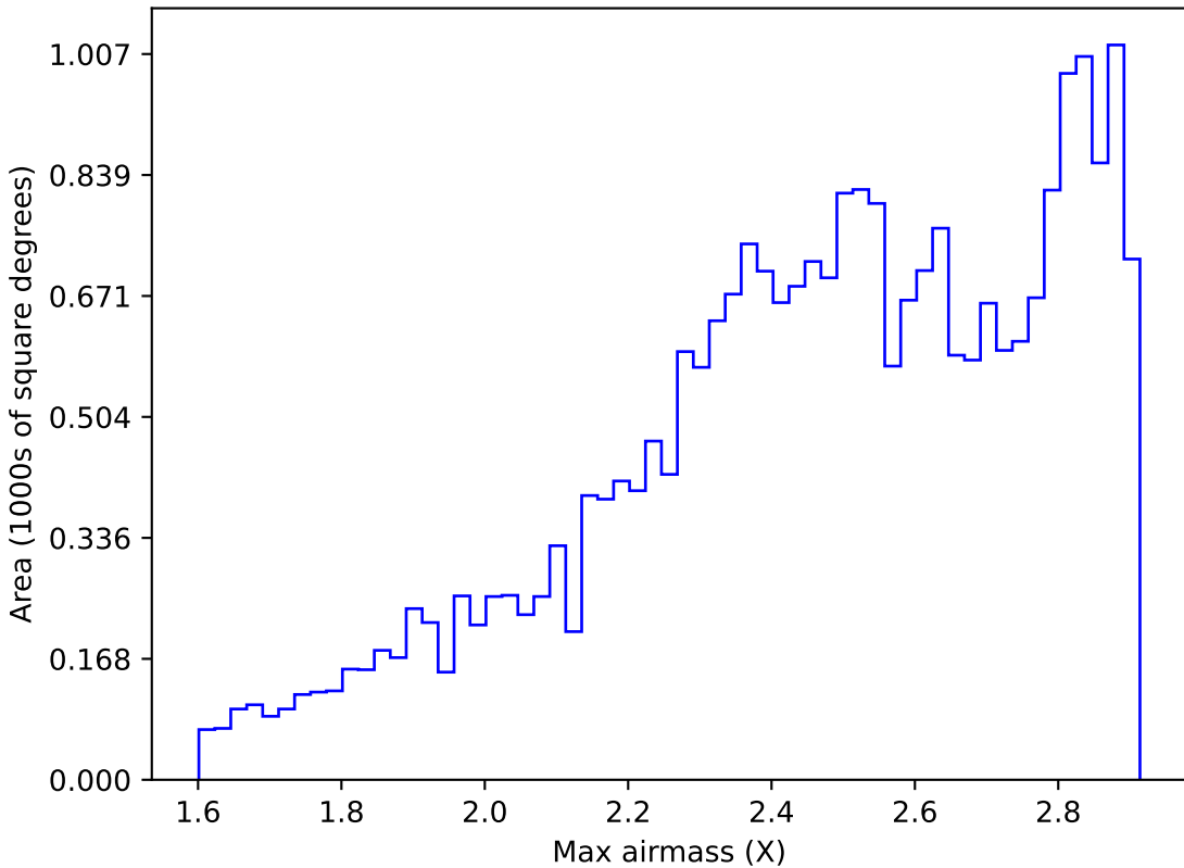
smc_lmc_v3.3_10yrs All sky z band: Max airmass
