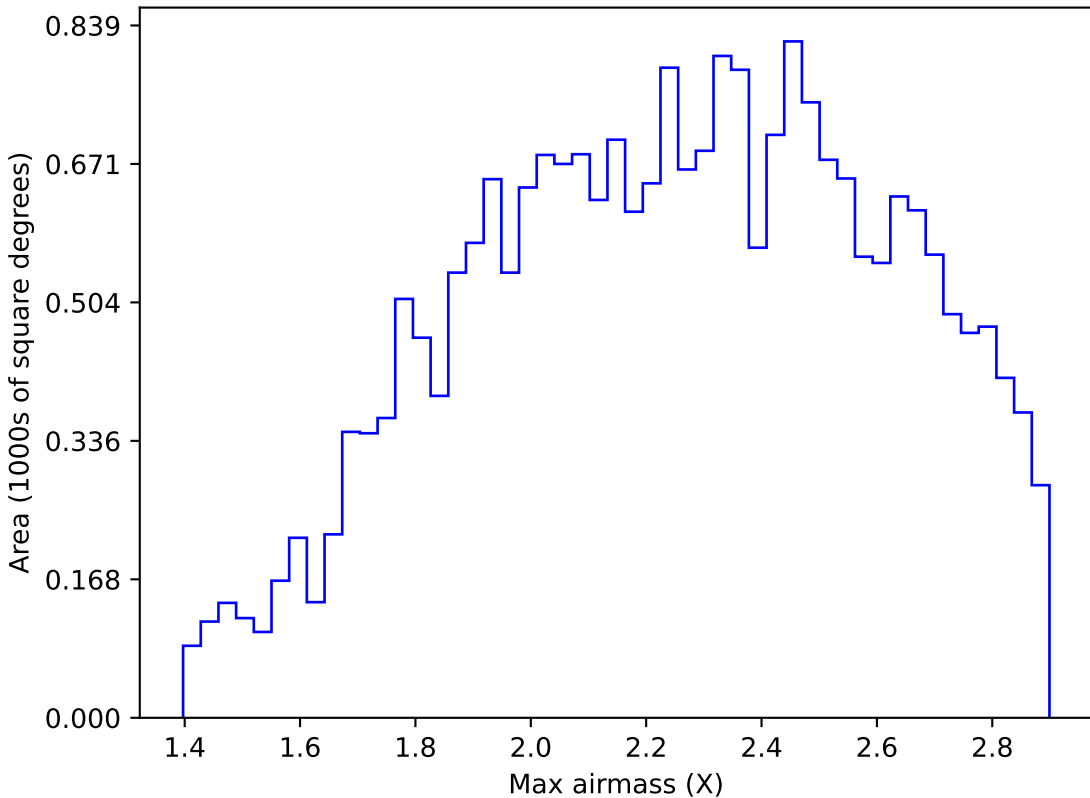
smc_lmc_v3.3_10yrs All sky y band: Max airmass
