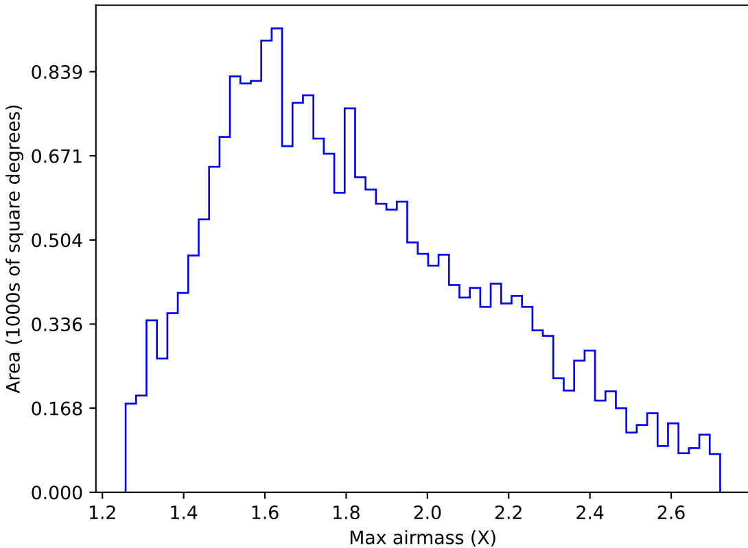
smc_lmc_v3.3_10yrs All sky u band: Max airmass
