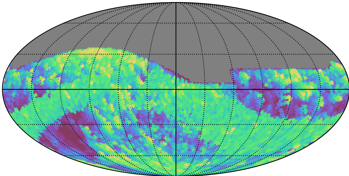
smc_lmc_v3.3_10yrs All sky r band: Max airmass
