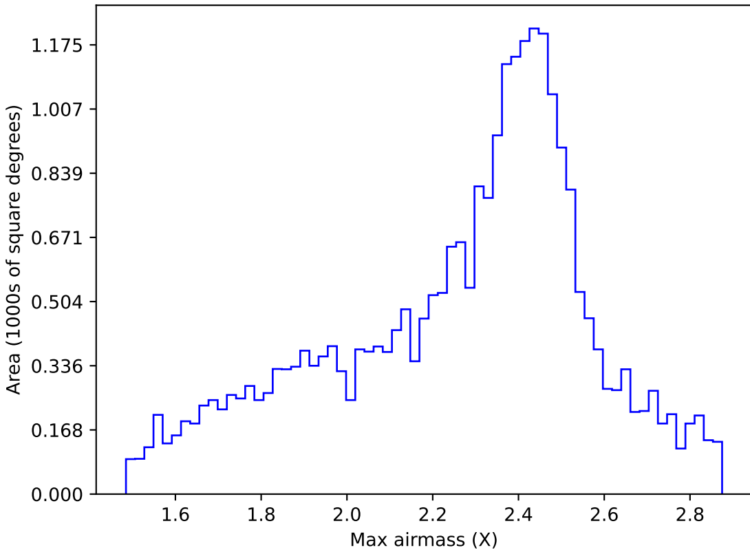
smc_lmc_v3.3_10yrs All sky r band: Max airmass
