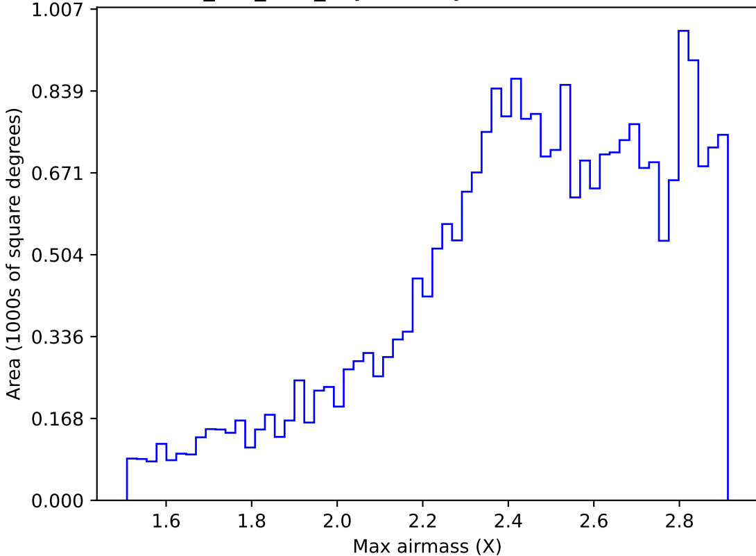
smc_lmc_v3.3_10yrs All sky i band: Max airmass
