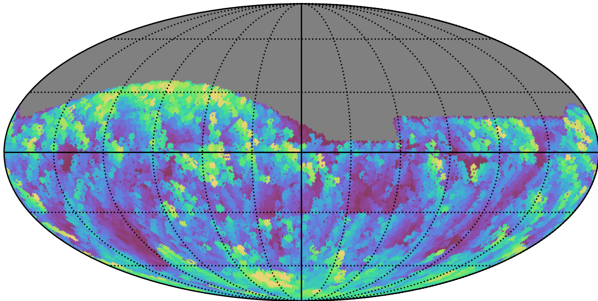
smc_lmc_v3.3_10yrs All sky g band: Max airmass
