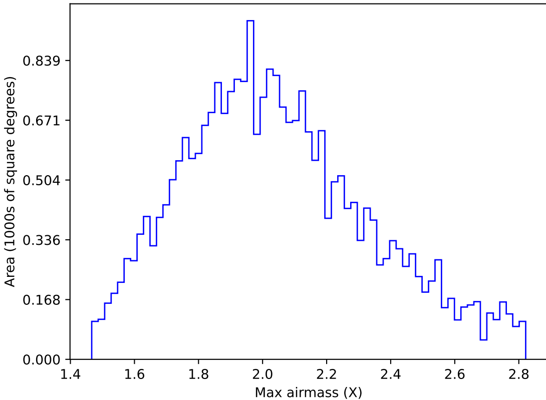
smc_lmc_v3.3_10yrs All sky g band: Max airmass
