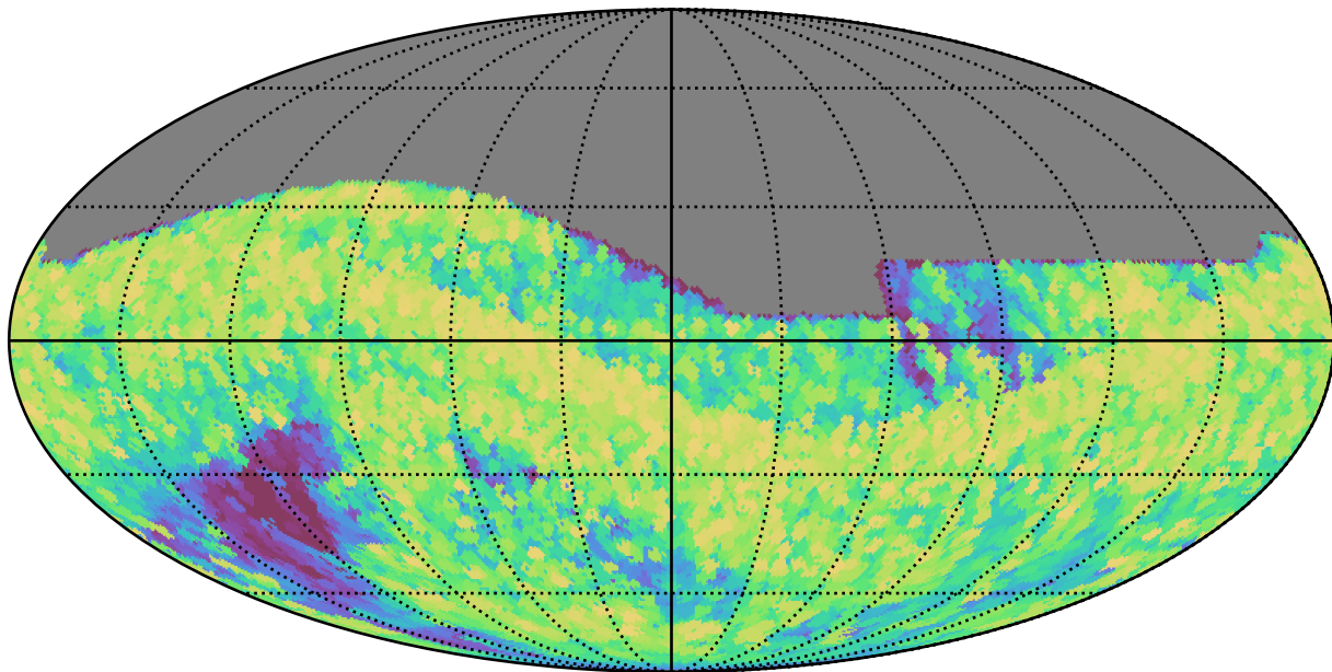
smc_lmc_v3.3_10yrs All sky all bands: Max airmass
