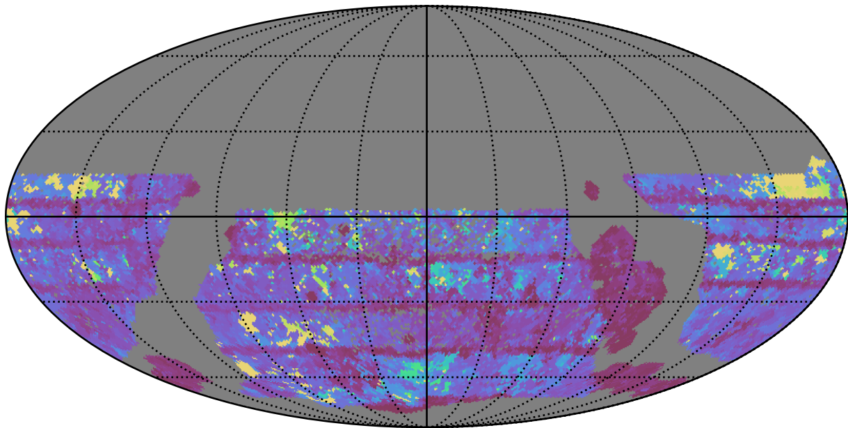
smc_lmc_v3.3_10yrs WFD z band: Max Inter-Night Gap
