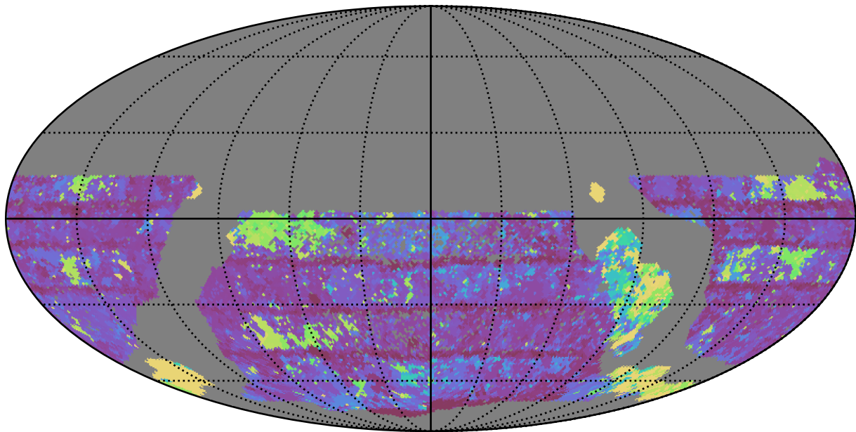
smc_lmc_v3.3_10yrs WFD y band: Max Inter-Night Gap
