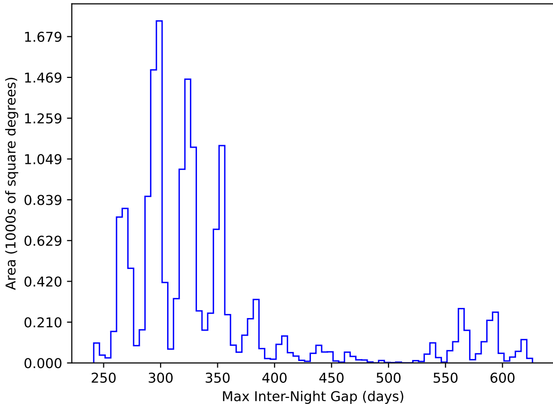
smc_lmc_v3.3_10yrs WFD y band: Max Inter-Night Gap
