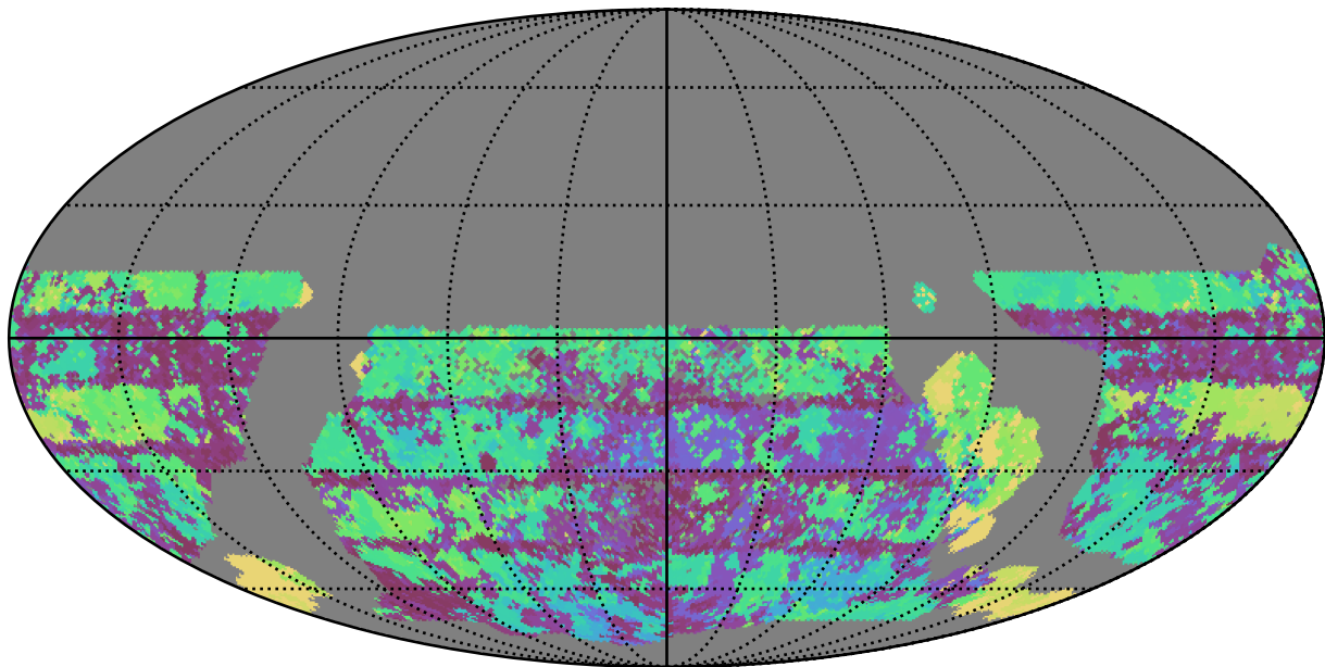
smc_lmc_v3.3_10yrs WFD u band: Max Inter-Night Gap
