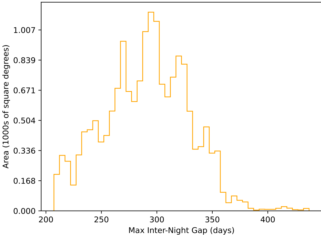
smc_lmc_v3.3_10yrs WFD r band: Max Inter-Night Gap
