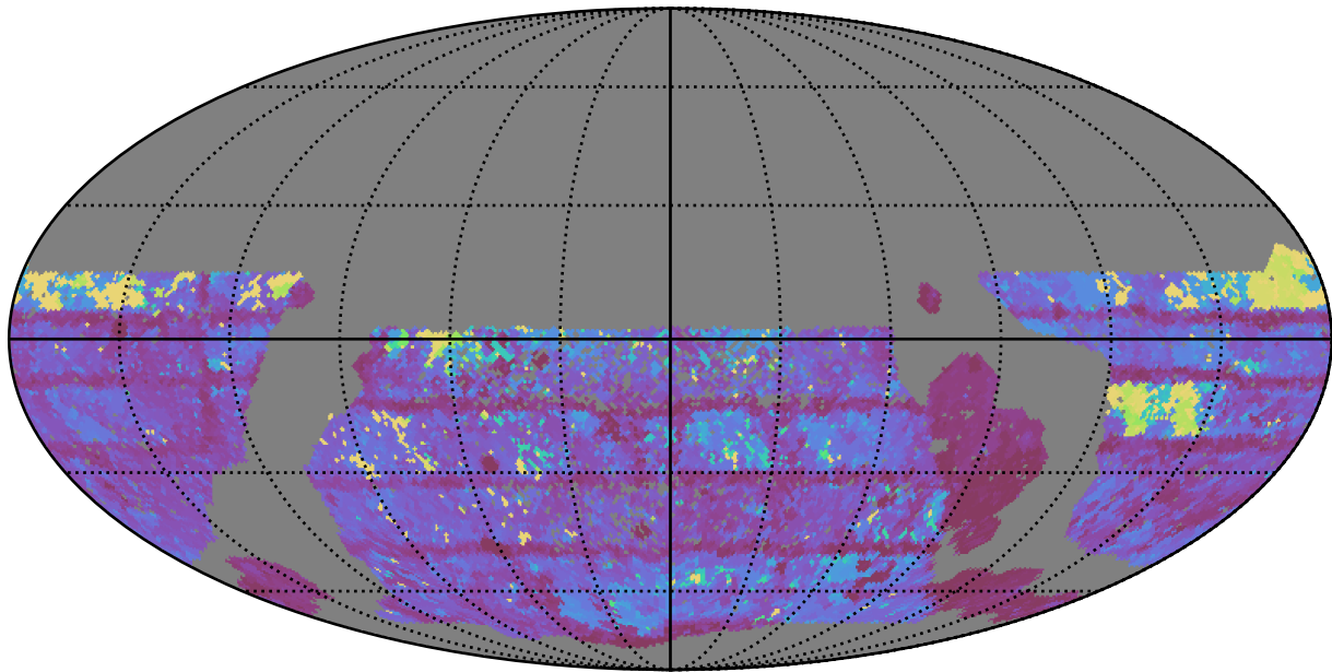
smc_lmc_v3.3_10yrs WFD i band: Max Inter-Night Gap
