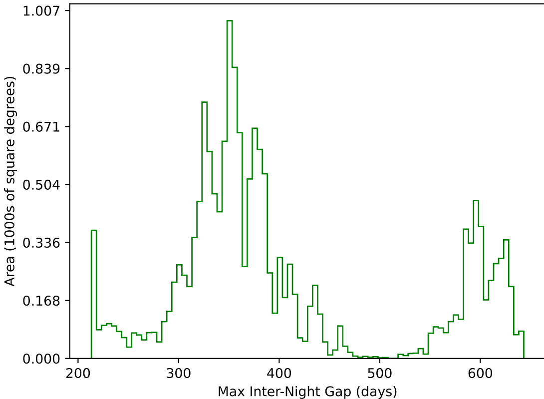
smc_lmc_v3.3_10yrs WFD g band: Max Inter-Night Gap
