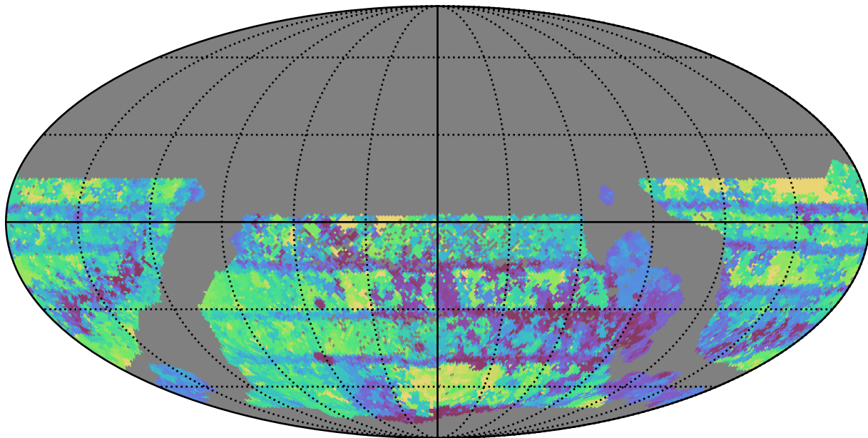
smc_lmc_v3.3_10yrs WFD all bands: Max Inter-Night Gap
