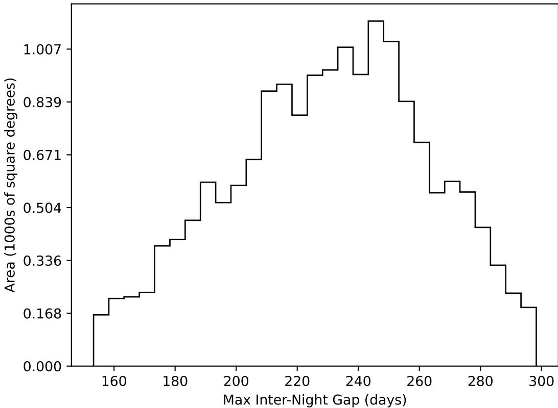
smc_lmc_v3.3_10yrs WFD all bands: Max Inter-Night Gap
