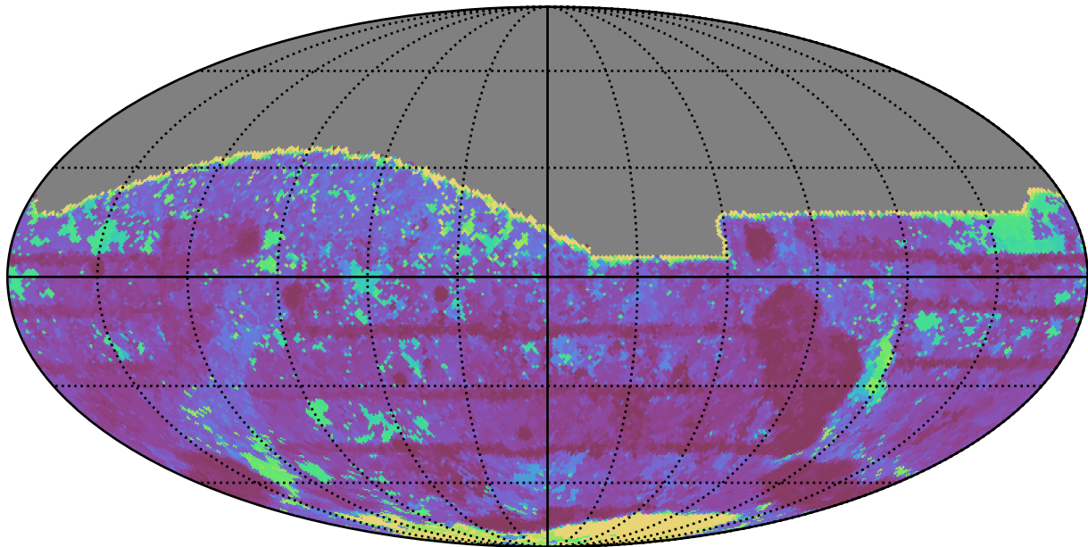
smc_lmc_v3.3_10yrs All sky z band: Max Inter-Night Gap
