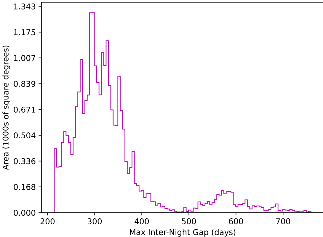
smc_lmc_v3.3_10yrs All sky z band: Max Inter-Night Gap
