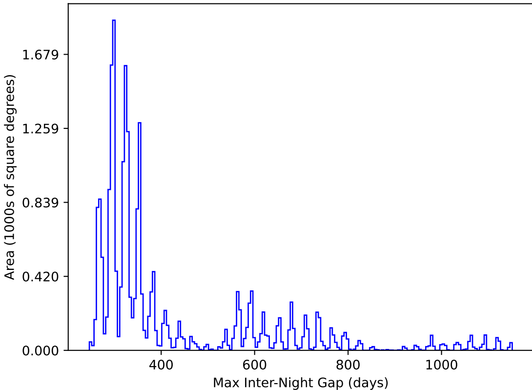
smc_lmc_v3.3_10yrs All sky y band: Max Inter-Night Gap
