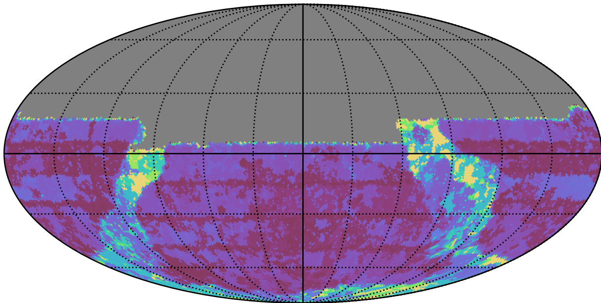
smc_lmc_v3.3_10yrs All sky u band: Max Inter-Night Gap
