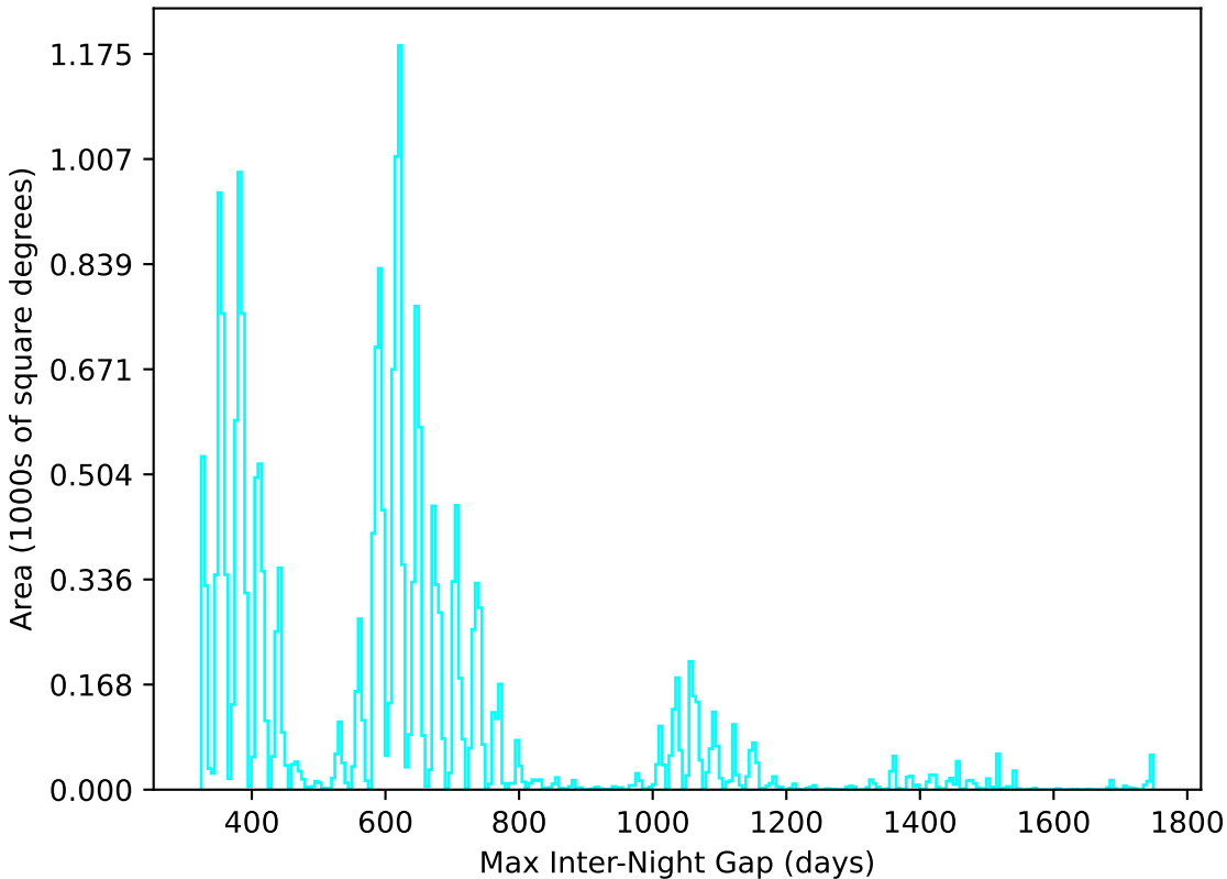
smc_lmc_v3.3_10yrs All sky u band: Max Inter-Night Gap
