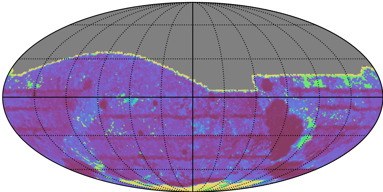
smc_lmc_v3.3_10yrs All sky r band: Max Inter-Night Gap
