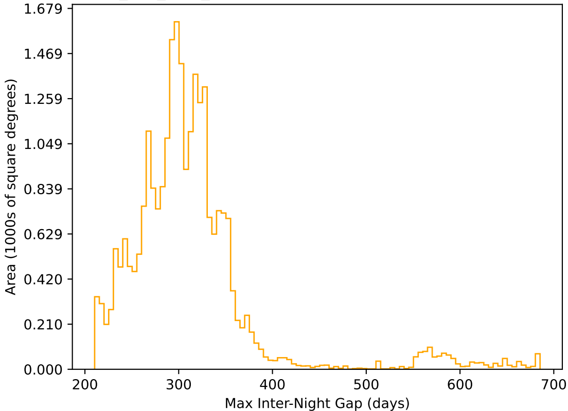
smc_lmc_v3.3_10yrs All sky r band: Max Inter-Night Gap
