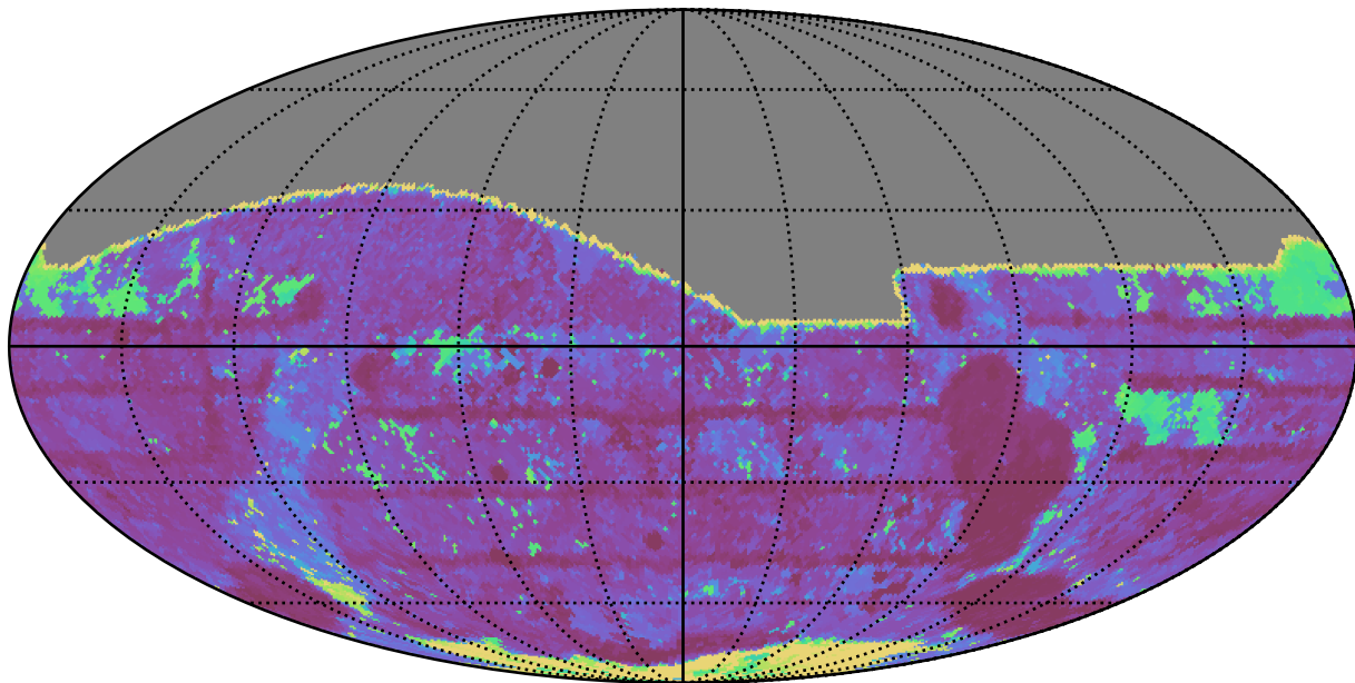
smc_lmc_v3.3_10yrs All sky i band: Max Inter-Night Gap
