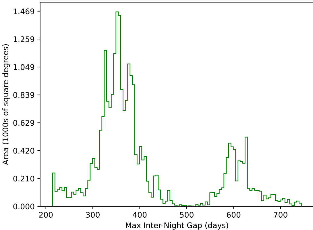
smc_lmc_v3.3_10yrs All sky g band: Max Inter-Night Gap
