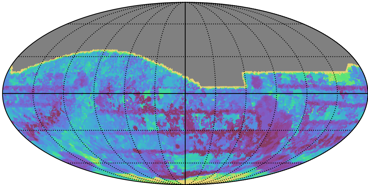
smc_lmc_v3.3_10yrs All sky all bands: Max Inter-Night Gap
