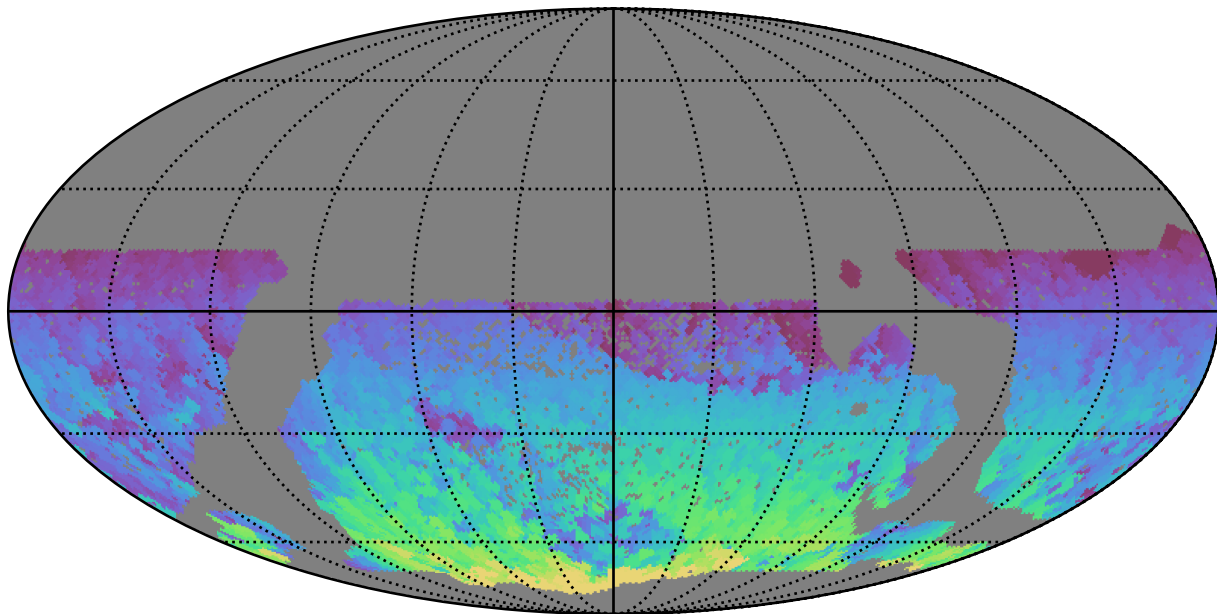
smc_lmc_v3.3_10yrs WFD z band: Max HA
