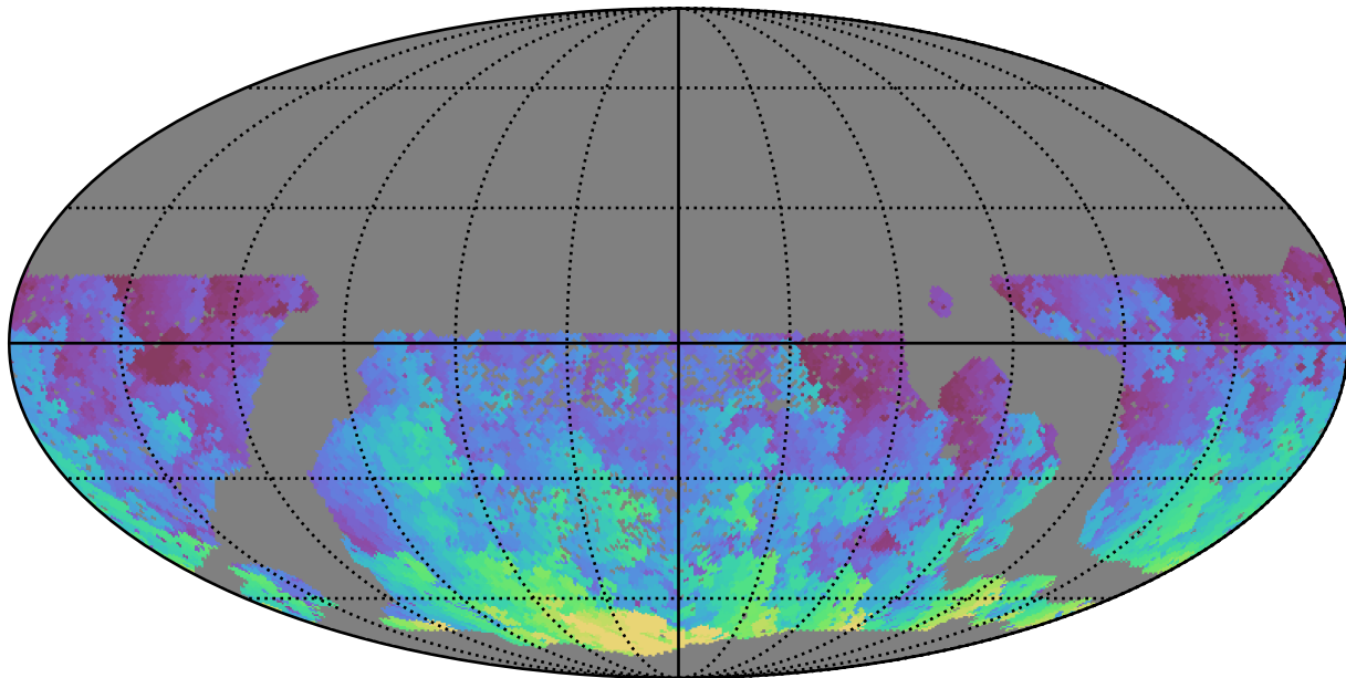
smc_lmc_v3.3_10yrs WFD u band: Max HA
