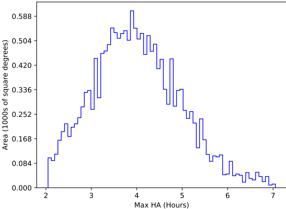
smc_lmc_v3.3_10yrs WFD u band: Max HA
