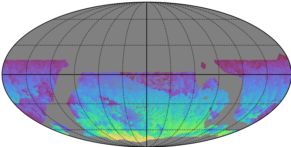
smc_lmc_v3.3_10yrs WFD i band: Max HA
