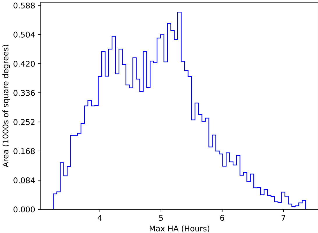
smc_lmc_v3.3_10yrs WFD i band: Max HA
