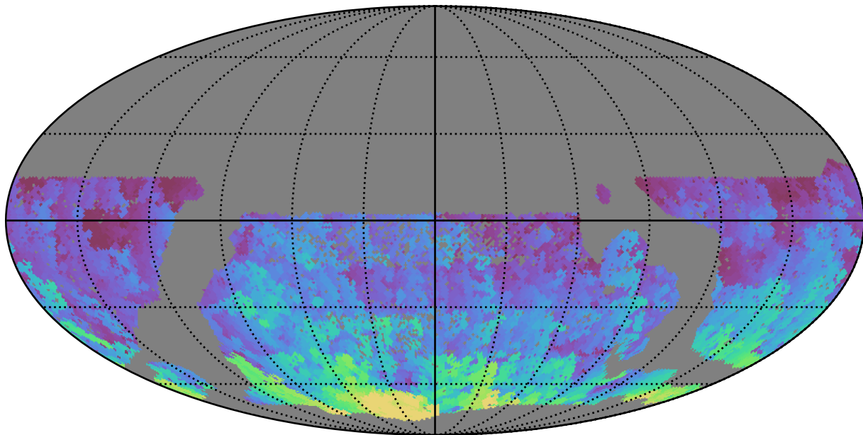
smc_lmc_v3.3_10yrs WFD g band: Max HA
