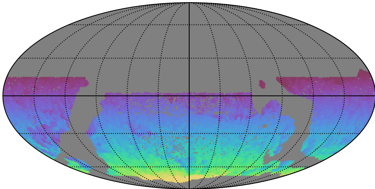
smc_lmc_v3.3_10yrs WFD all bands: Max HA
